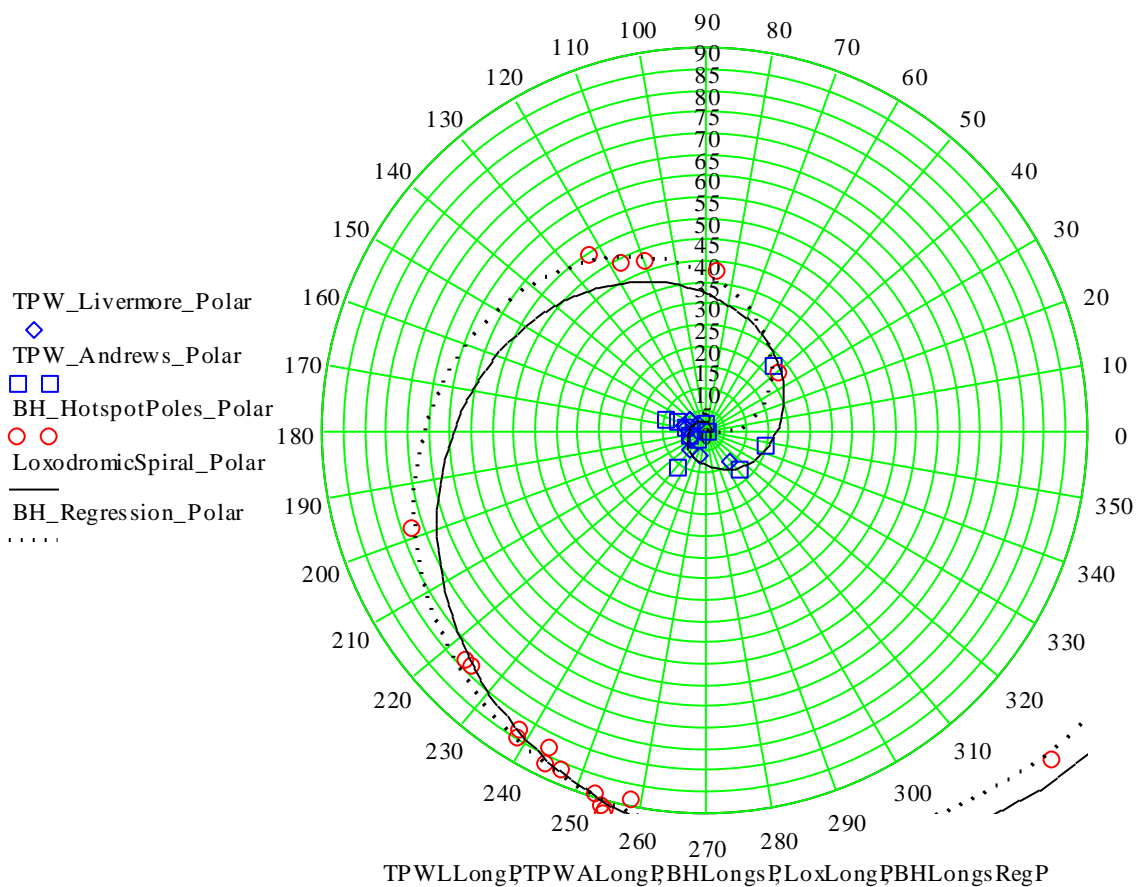
Loxodromic (solid) and Linear (dashed) CCW Spirals Fit to TPW [Livermore,1984; Andrews,1985] and the "B+H" Hotspot Poles (only "B" Poles showing)
