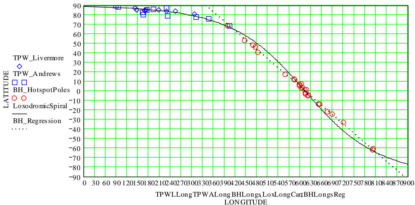
Loxodromic (solid) and Linear (dashed) CCW Spirals Fit to TPW [Livermore,1984; Andrews,1985] and the "B+H" Hotspot Poles
